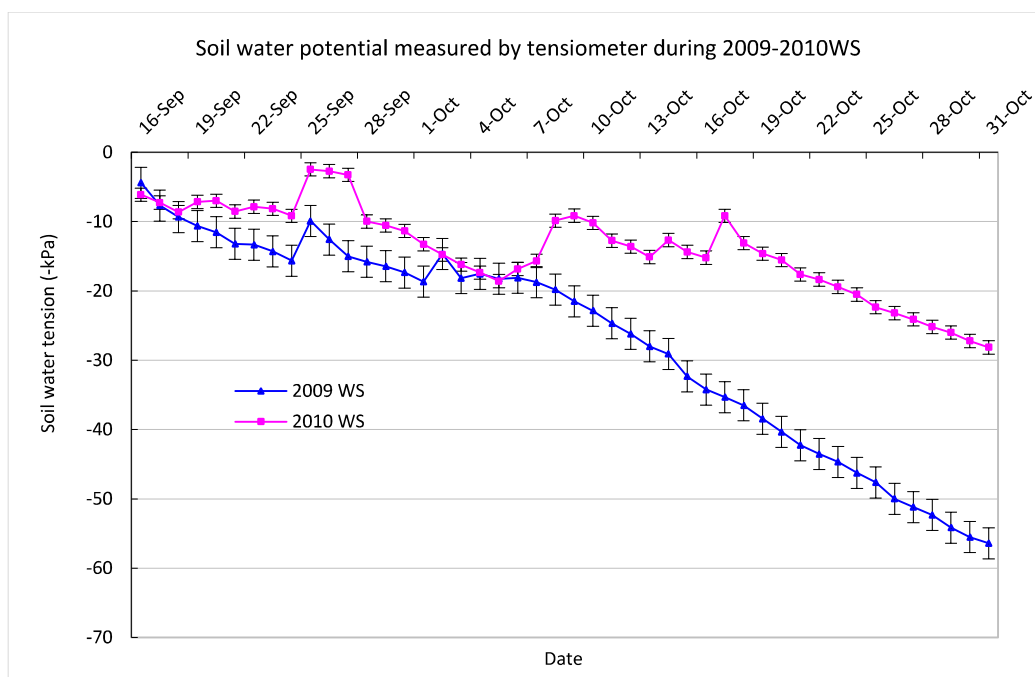
Fig. 5. Soil water potential at the experimental fields during 2009WS and 2010WS at Godagari, Rajshahi, Bangladesh.
